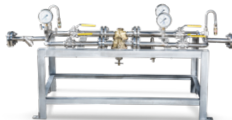
双路调压装置 (Rego调压阀) dual way pressure regulating device(REGO regulate valve)
